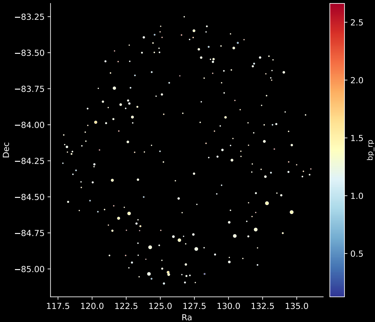
APOGEE DR17 Field: [301-33-C] Stars: 221
