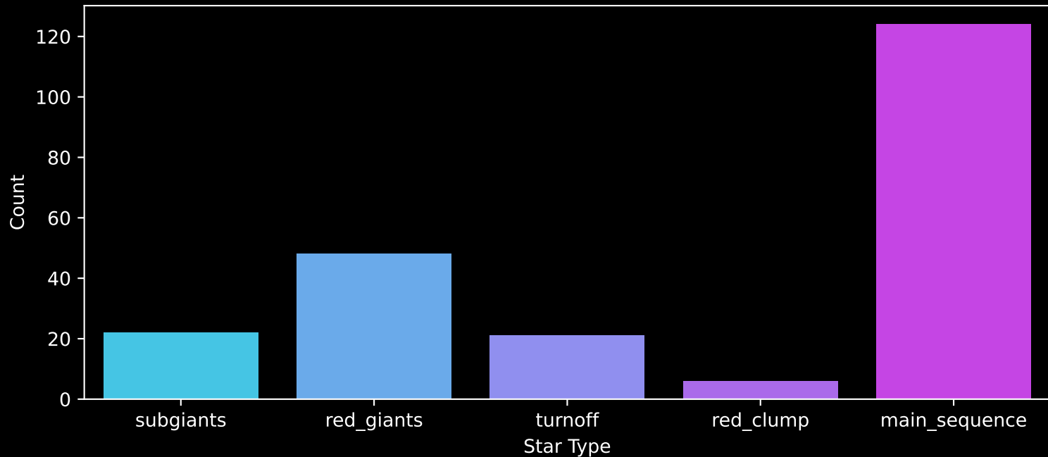
APOGEE DR17 Field: [301-33-C] Count plot of Star Type
