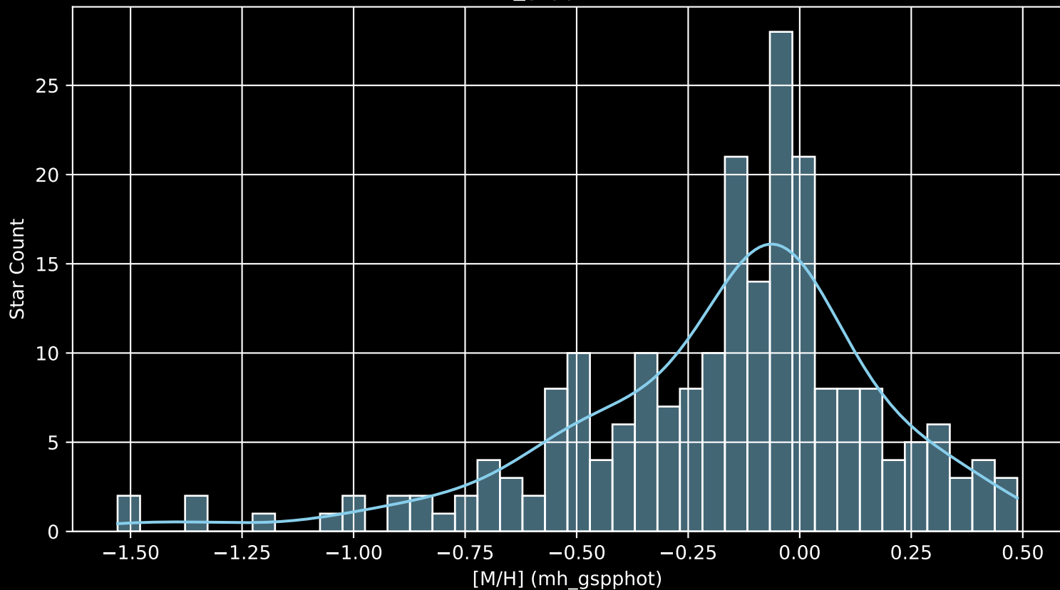
APOGEE DR17 Field: [301-33-C [M/H] (mh_gspphot) (n= 220)
