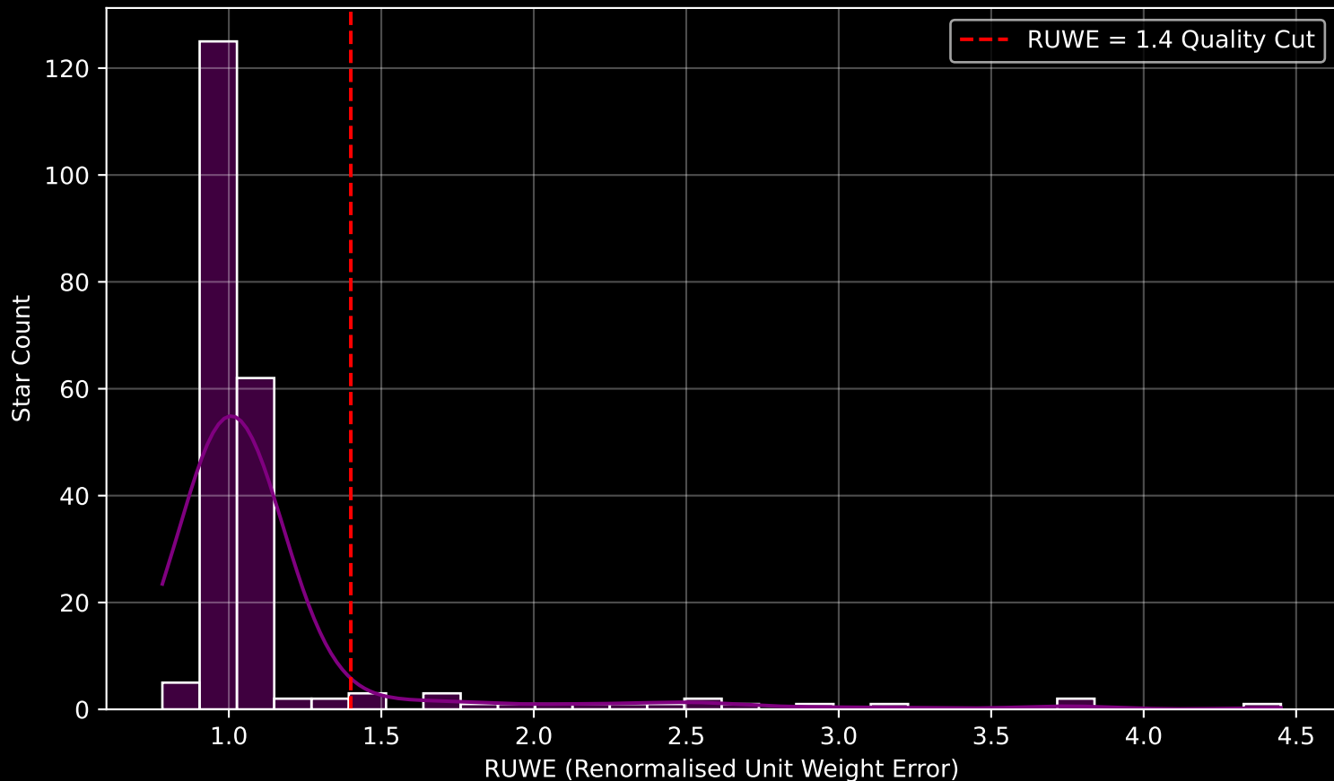
GAPOGEE DR17 Field [301-33-C] RUWE Distribution (n= 216)
