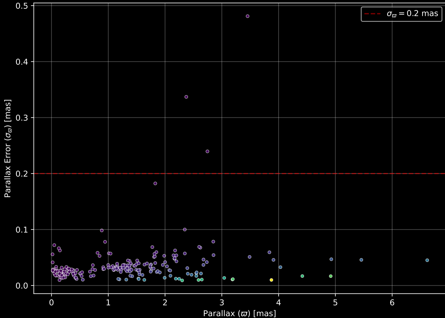
APOGEE DR17 Field: [301-33-C] Parallax Quality (n= 221)
