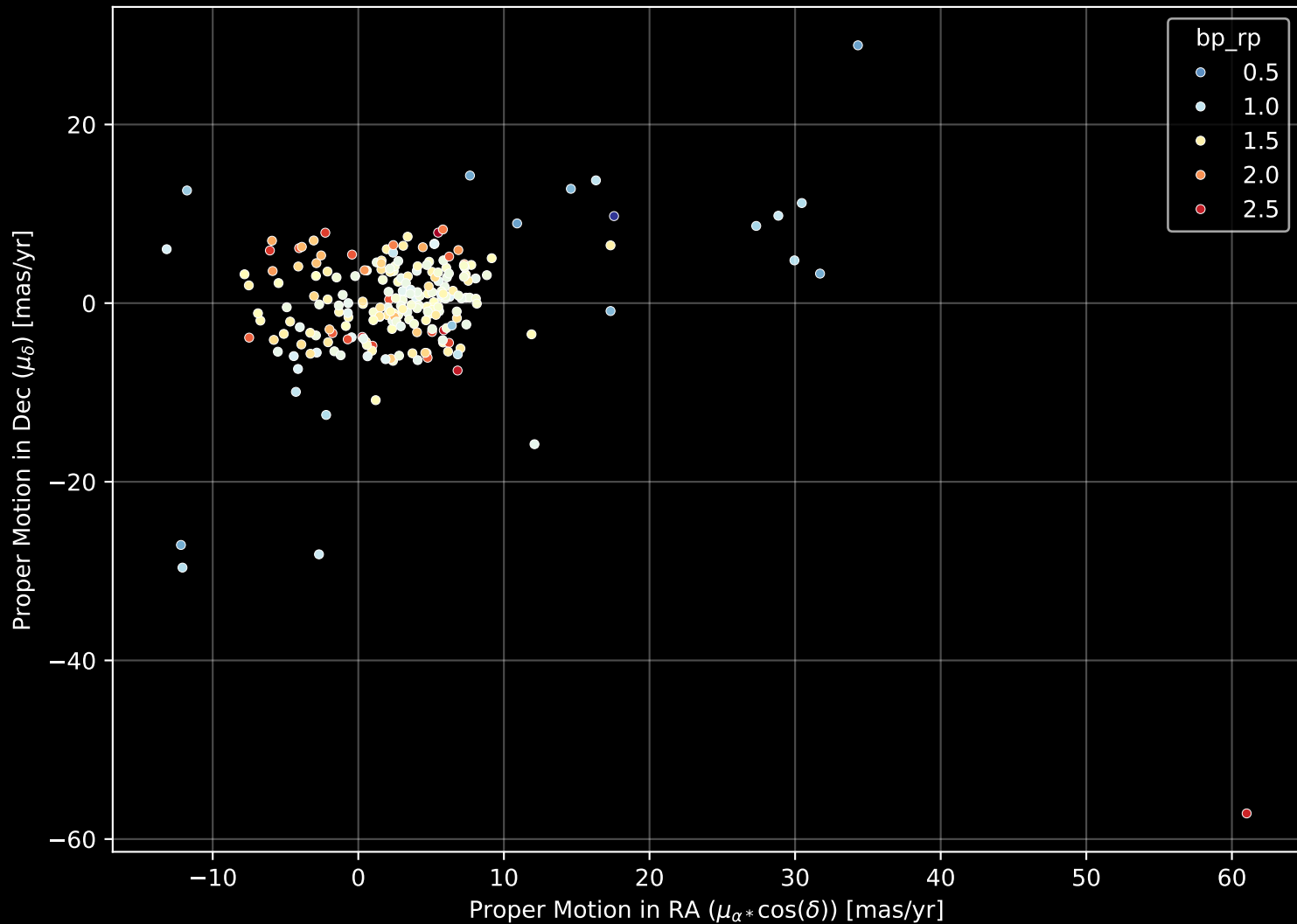
APOGEE DR17 Field: [301-33-C] Proper Motion Diagram (n= 221)
