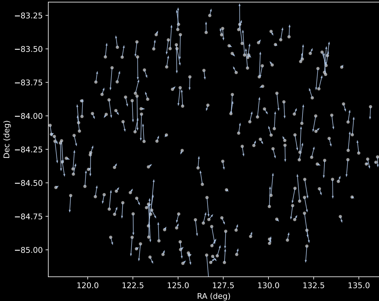
APOGEE DR17 Cluster 1 Proper Motion Vectors (n=210)
